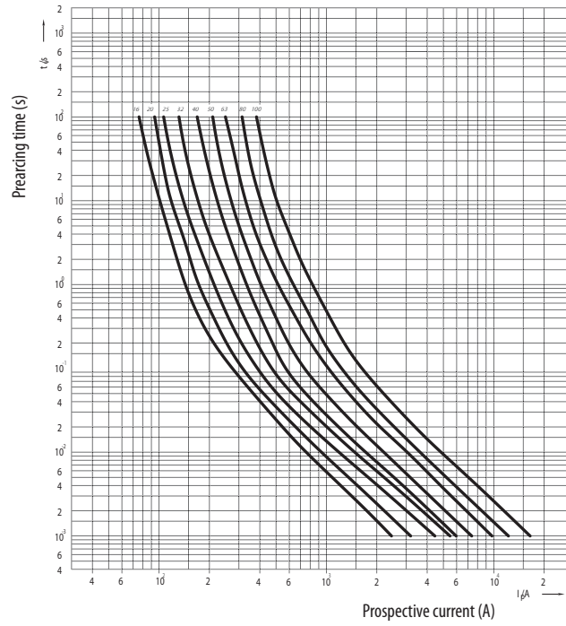
Time current characteristics I/t, aM CH10, 14, 22
