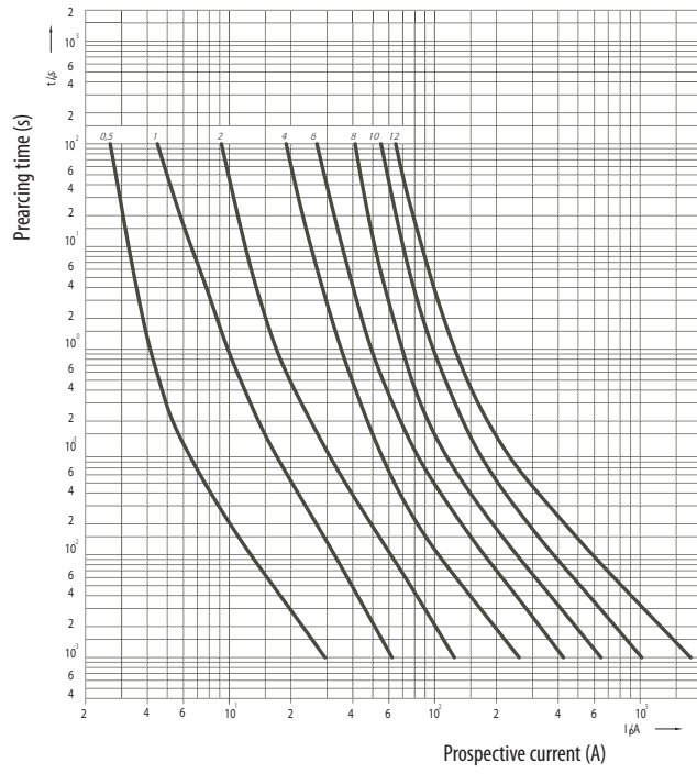
Time current characteristics I/t, aM CH10, 14, 22
