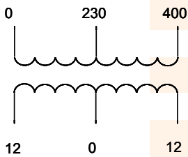
Single phase safety transformers Primary voltage 230, 400V. Secondary voltage 24V (12V-0-12V). Thermal class B
