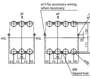
Drilling plan (front view)
